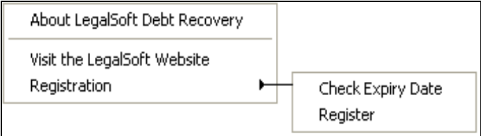
Figure 2. Help Menu.
